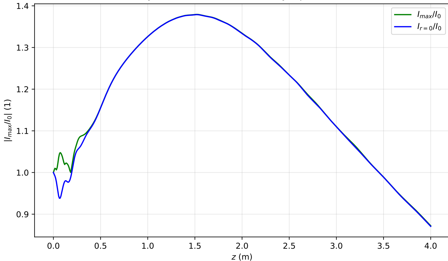
I_{max}(x = 0, y = 0, z)/I_0 , P_{in}=0.8P_{cr} , noisy input, artificial time
